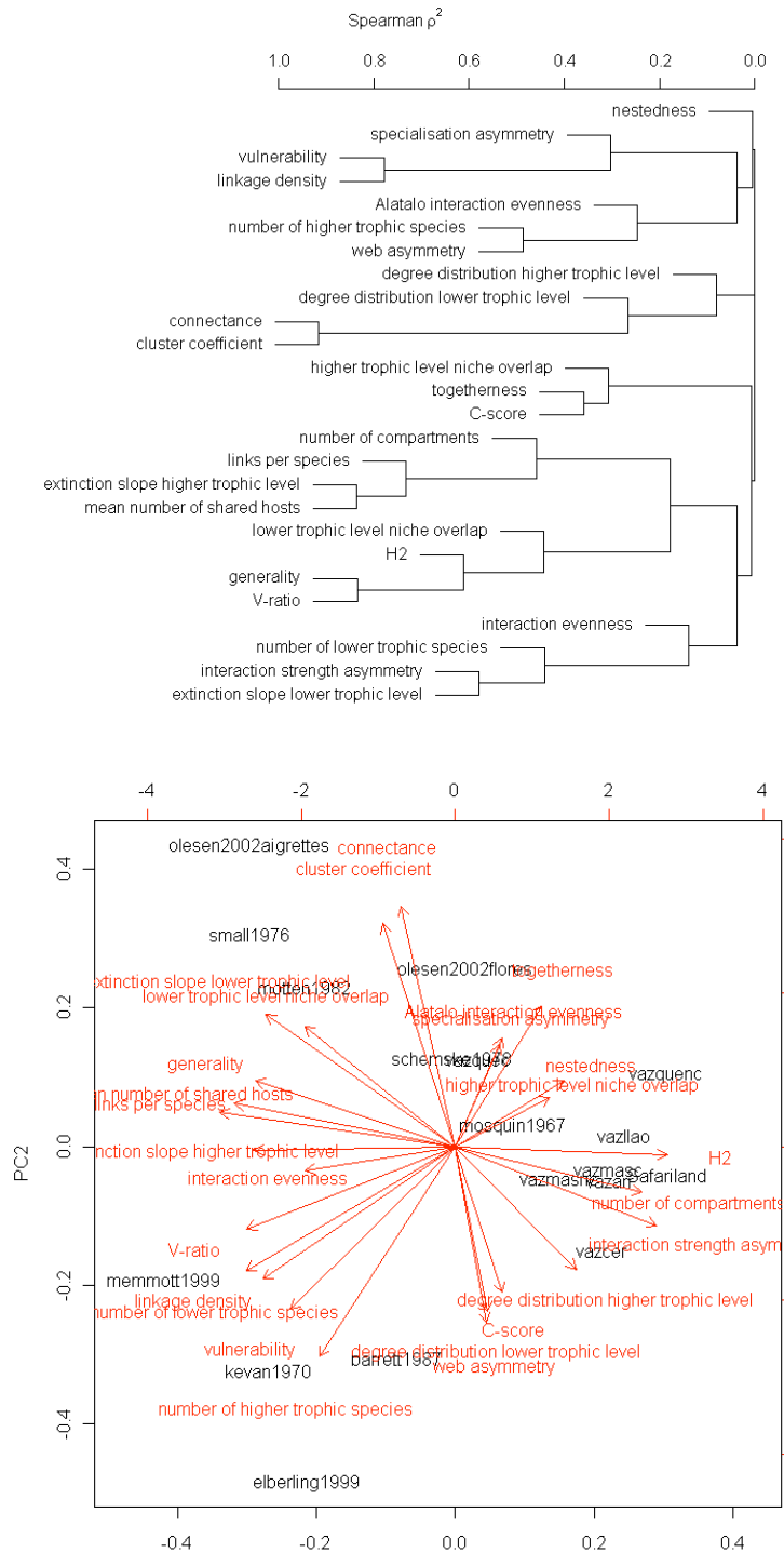
Fig. (5). Relationship between indices of the observed pollination networks as depicted in a cluster analysis (top: distance based on squared Spearman's rank correlation coefficient) and a PCA (bottom). These two-dimensional representations hide the fact that variables plotted here as distant may well be correlated in other dimensions. In both cases the large network of Kato et al. (1990) was omitted, because it distorts the presentation (although not the outcome: see Fig. (S5)).
